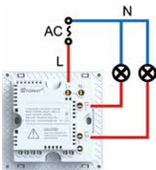
Connection 1: Without neutral wire
