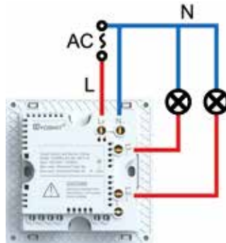
Connection 2: With neutral wire
